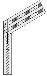
D3 ROOF EXTERNAL WALL JOINT
