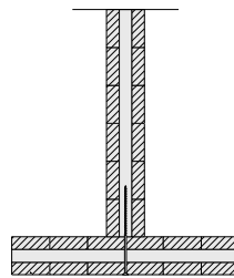
D8 T-WALL JOINT
