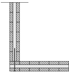
D7 CORNER WALL JOINT
