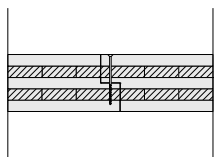
D10 FLOOR/ROOF PANEL JOINT
