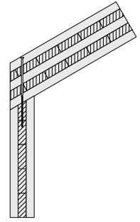
D3 ROOF EXTERNAL WALL JOINT
