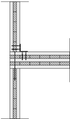
D4 FLOOR EXTERNAL WALL JOINT
