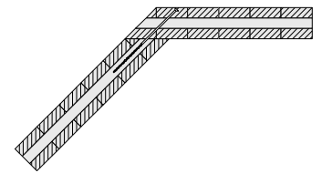
D9 ANGLE WALL JOINT
