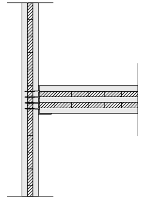
D6 FLOOR INTERNAL WALL JOINT (CONTINUOUS)
