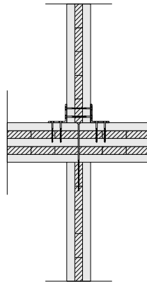
D5 FLOOR INTERNAL WALL JOINT
